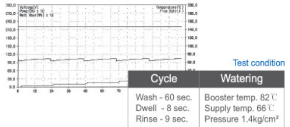
Temperature test
